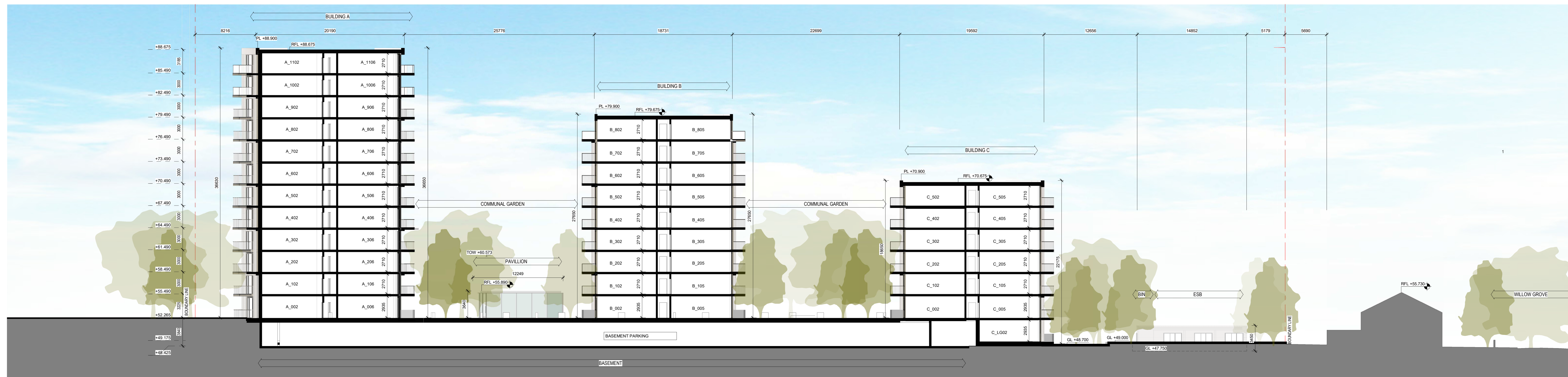
1 SECTION BUILDINGS A B C 1 : 200
